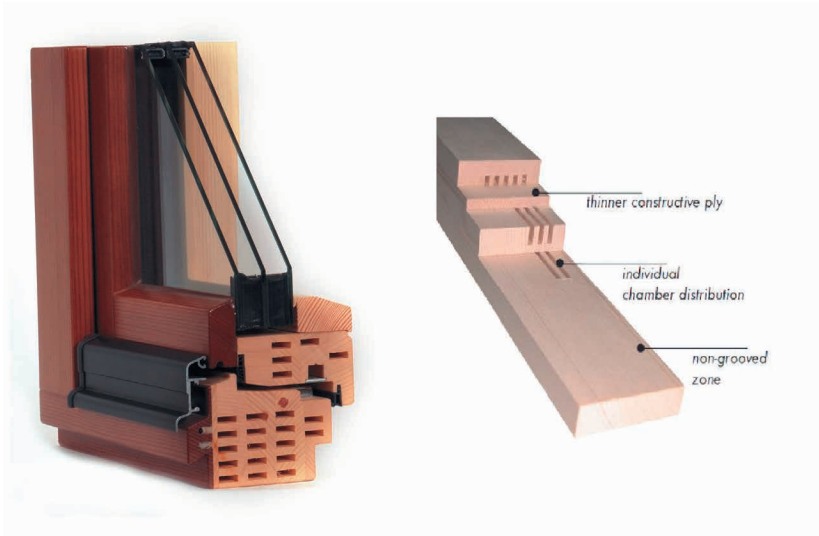
Foto 4.7. AiroTherm.
