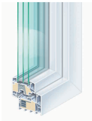
Figura 3.3. Sistema 88plus proEnergyTec (KÖMMERLING).
