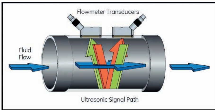
Transit-time flow measurement technique
